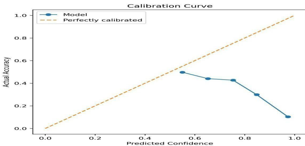
Figure 5.3: Calibration Curve
